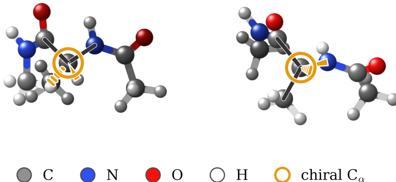
Figure 21: The two enantiomers of alanine dipeptide: the energy-minimized L-form and the D-form, a 3D reflection of it, shown from different viewpoints (ball-and-stick; C grey, N blue, O red, H white). The chiral C_\alpha is ringed in gold with stereo bonds, a solid wedge toward the viewer and hashed bonds behind. The achiral Amber force field makes the two isoenergetic, so the generator emits both, the structural companion to the (\phi, \psi) \rightarrow (-\phi, -\psi) Ramachandran symmetry of Fig. 22.
