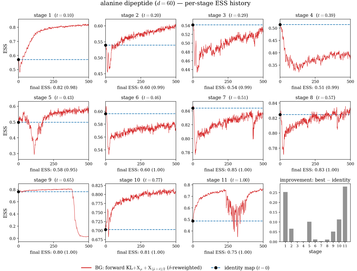
Figure 19: Alanine dipeptide per-stage ESS history: each panel is the per-step effective sample size during that stage’s X-regularized \delta -reweighted flow training (red), against the identity-map baseline at t = 0 (blue dashed). Below each panel is that stage’s accepted validation ESS with the sharpening ESS in parentheses. The dip across t \approx 0.29 – 0.46 is the clash bottleneck, with ESS recovering to \approx 0.8 once the cap is sharp enough to separate the basins.
