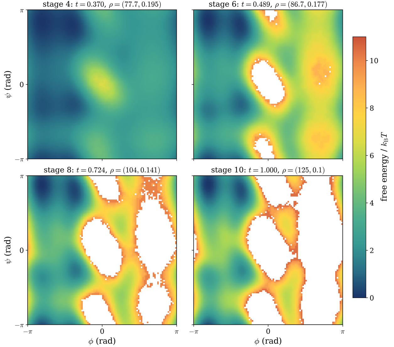
Figure 13: Alanine dipeptide Ramachandran free energy surfaces at accepted stages 4, 6, 8, and 10. Each panel contains 10^7 inference samples obtained by generating pushforward samples with the corresponding stage flow and then applying resampling, rejuvenation, sharpening, and post-sharpen rejuvenation. The panel titles give the interpolation parameter and regularization value; stage 10 reaches t = 1 and \rho = (125, 0.10) . A common colorbar reports free energy relative to the observed minimum in units of k_B T .
