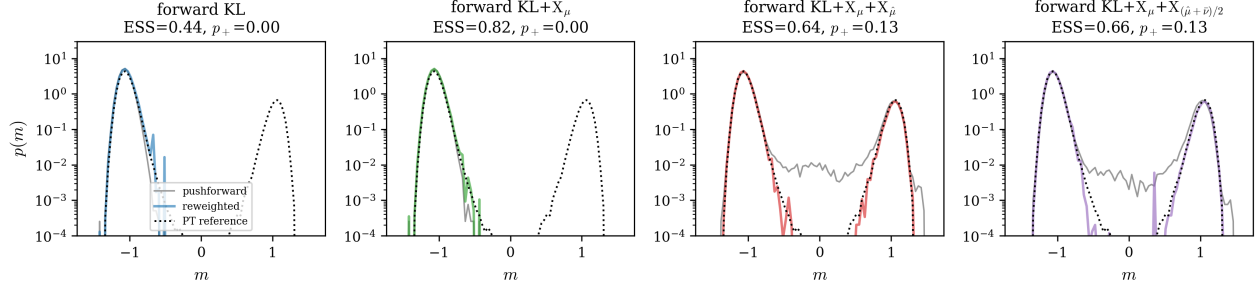
Figure 7: Magnetization distribution p(m) at L = 8 for the four losses: pushforward (gray), reweighted (color), PT reference (dotted). Titles report the final ESS and the reweighted p_+ . Forward KL and KL+ X_\mu match the favored vacuum beautifully and miss the m > 0 phase entirely; the oracle-driven losses recover both peaks at the correct relative weight.
