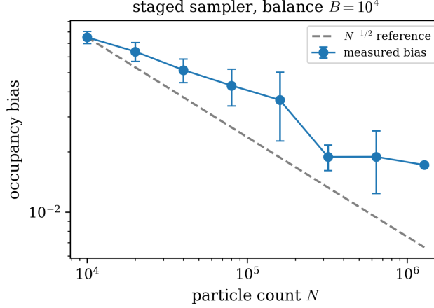
Figure 9: Occupancy bias \frac{1}{6} \sum_s |p_s - \frac{1}{6}| of fresh staged rebuilds through the trained B = 10^4 ladder of the X-regularized loss, versus rebuild size N = 10^4 \cdot 2^k , k = 0, \dots, 7 , averaged over 2^{7-k} independent rebuilds per size at equal total work; error bars are \pm 2 standard errors. The bias decays steadily but slower than the dashed Monte Carlo reference N^{-1/2} , at the log-log slope -0.34 : the six composed resampling steps correlate the surviving lineages, and the resampling error compounds across stages.
