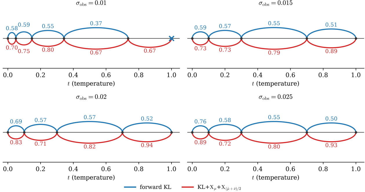
Figure 11: ESS ladders on the screened Poisson posterior across the noise sweep, one panel per \sigma_{\text{obs}} . The temperature axis runs t = 0 \rightarrow 1 ; each accepted stage is an arc spanning its increment \Delta t_k , forward KL above (blue) and the X-regularized loss \text{KL} + X_\mu + X_{(\hat{\mu} + \bar{\nu})/2} below (red), labelled by its per-stage validation ESS. The cross marks the final bridge that the forward KL run failed in all ten attempts at \sigma_{\text{obs}} = 0.01 . The recovered well weights are reported in Table 7.
