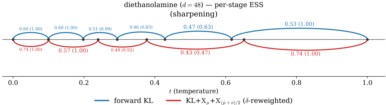
Figure 14: Diethanolamine per-stage ESS as annealing-ladder arcs (sharpening schedule): forward KL above the axis (blue), \text{KL} + \text{X}_\mu + \text{X}_{(\hat{\mu} + \bar{\nu})/2} , \delta -reweighted, below (red). Each arc is an accepted stage; the apex label is that stage’s validation ESS, with the sharpening ESS in parentheses.
