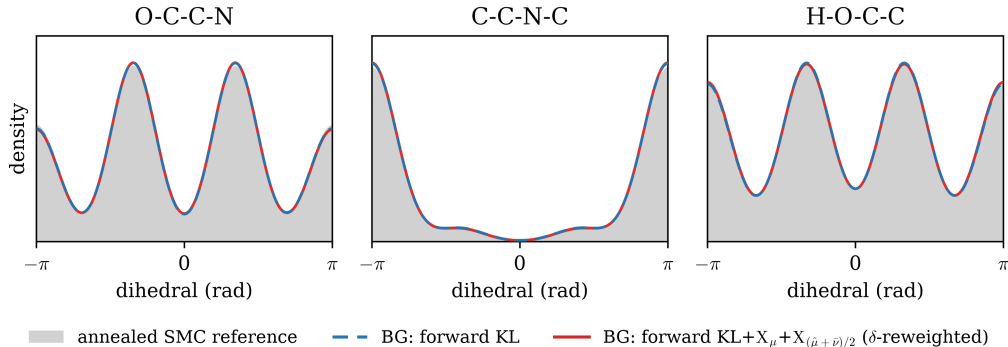
Figure 15: Diethanolamine torsion marginals of both generators against a converged annealed SMC reference (grey): forward KL (blue) and \text{KL} + X_\mu + X_{(\hat{\mu} + \bar{\nu})/2} , \delta -reweighted (red), both sharpened with the cap annealed to e_{\text{cap}} = 200 kJ/mol. Both recover the multimodal backbone torsions and track the annealed SMC reference.
