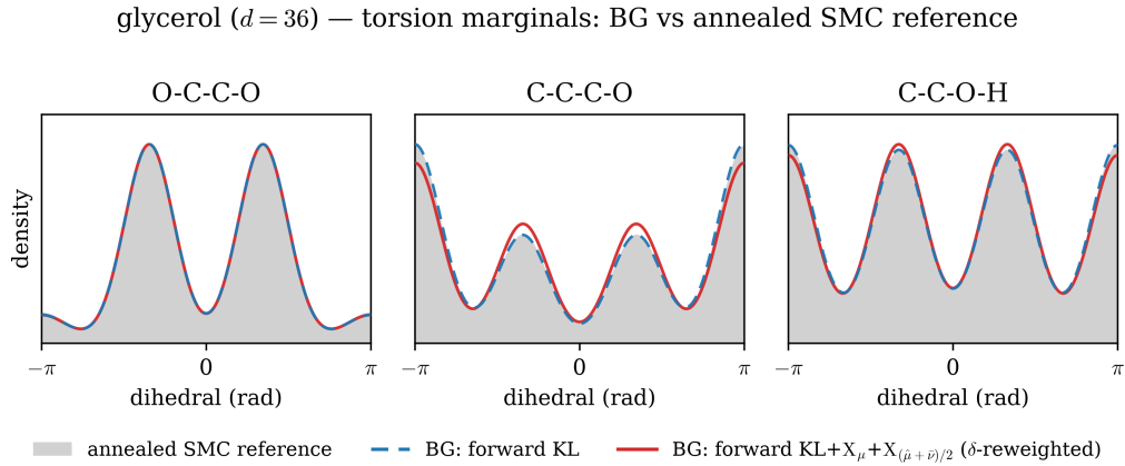
Figure 13: Glycerol torsion marginals of both generators against a converged annealed SMC reference (grey): forward KL (blue) and \text{KL} + X_\mu + X_{(\hat{\mu} + \bar{\nu})/2} , \delta -reweighted (red), both sharpened with the cap annealed to e_{\text{cap}} = 200 kJ/mol. Both recover the multimodal gauche ^\pm /trans structure of the characteristic glycerol torsions.
