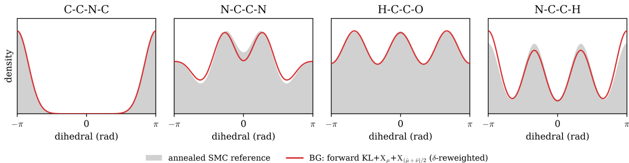
Figure 17: Alanine dipeptide torsion marginals of the BG deliverable (red) against a converged annealed SMC reference (grey). The four most multimodal proper torsions are shown; the densities are \pm\phi -symmetrised, the achiral target having p(\phi) = p(-\phi) . The BG recovers the multimodal backbone torsions and tracks the reference; the peptide-bond torsion \omega (C-C-N-C) is trans-dominant in the generator, the one torsion whose high rotation barrier also makes the uniform-init annealed SMC reference slow to converge.
