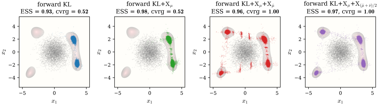
Figure 3: Himmelblau target. Columns show forward KL, \text{KL}+X_\mu , \text{KL}+X_\mu+X_{\hat{\mu}} , and \text{KL}+X_\mu+X_{(\hat{\mu}+\bar{v})/2} ; each panel shows the pushforward samples over the target energy with final ESS and coverage, and gray points show the source. The first two objectives capture only two of the four wells. Both \hat{\mu} -weighted objectives cover all four, while including pushforward samples in the mixture term reduces the visible intermodal mass and raises ESS relative to the \text{KL}+X_\mu+X_{\hat{\mu}} fit.
