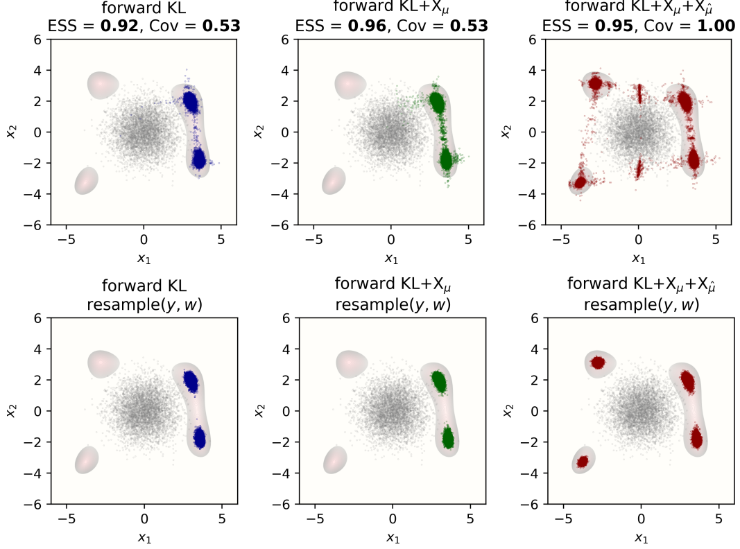
Figure 1: Himmelblau target. Row 1: pushforward y = G^{-1}(x) . Row 2: resample( y, w ) with Langevin rejuvenation. Columns: forward KL, forward KL + X_\mu , forward KL + X_\mu + X_{\hat{\mu}} . Each pushforward panel title reports the final ESS and the k = 5 coverage of the QT-generated \hat{\mu} .
