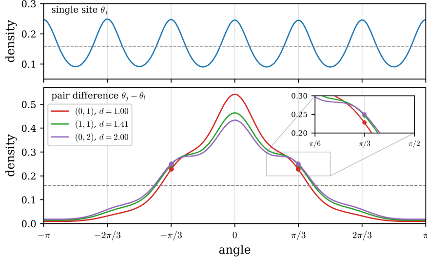
Figure 8: Angle densities from 2 \times 10^6 fresh samples advanced through the trained B = 2000 \text{KL} + \text{X}_\pi + \text{X}_{(\hat{\pi} + \bar{\nu})/2} stage sequence by map, reweighting, resampling, and MALA. The upper panel is the single-site marginal. The lower panel gives pair differences at offsets (0, 1) , (1, 1) , and (0, 2) ; dots and the inset resolve the one-clock-step angle \pi/3 . Dashed lines show the uniform density.
