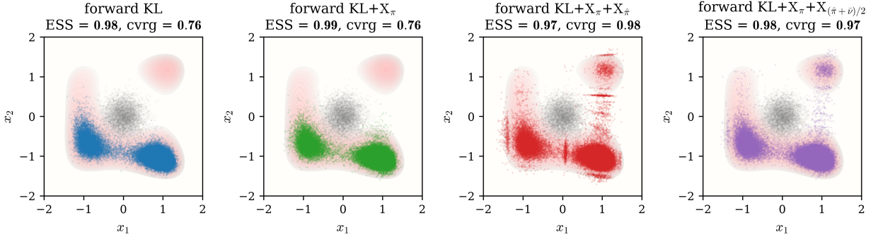
Figure 3: Three-Well target. From left to right, the panels show forward KL, \text{KL}+X_\pi , \text{KL}+X_\pi+X_{\hat{\pi}} , and \text{KL}+X_\pi+X_{(\hat{\pi}+\bar{\nu})/2} . Each panel overlays the pushforward samples on the target energy and reports final ESS and coverage; gray points show the source.
