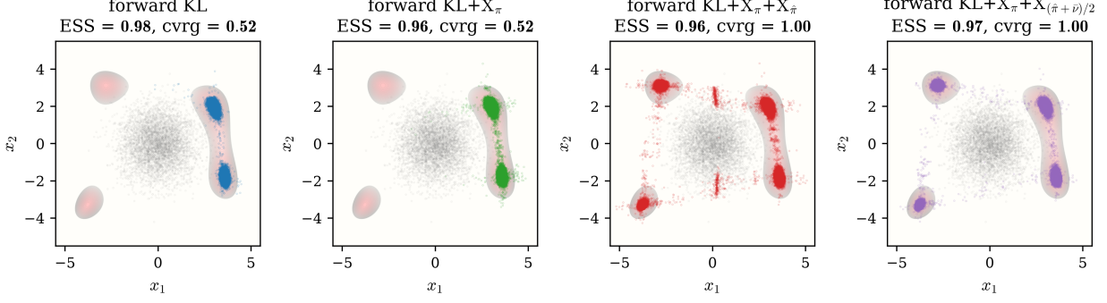
Figure 4: Himmelblau target. Columns show forward KL, \text{KL}+X_\pi , \text{KL}+X_\pi+X_{\hat{\pi}} , and \text{KL}+X_\pi+X_{(\hat{\pi}+\bar{\nu})/2} ; each panel shows the pushforward samples over the target energy with final ESS and coverage, and gray points show the source.
