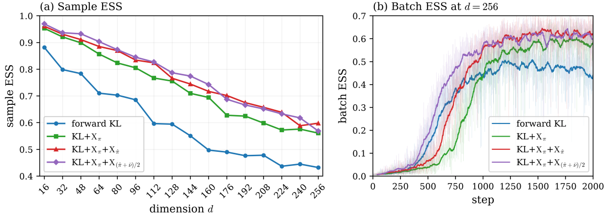
Figure 6: ESS on the product multi-well target (30). (a) Final sample ESS over sixteen tested dimensions. (b) Batch ESS during the d = 256 training; bold curves are 40-step moving averages of the raw values.
