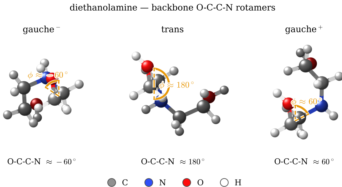
Figure 17: Typical diethanolamine configurations at the three states of a backbone O-C-C-N torsion: gauche − ( -60^\circ ), trans ( 180^\circ ), gauche + ( +60^\circ ). The gold arc marks the dihedral \phi ; ball-and-stick (C grey, N blue, O red, H white).
