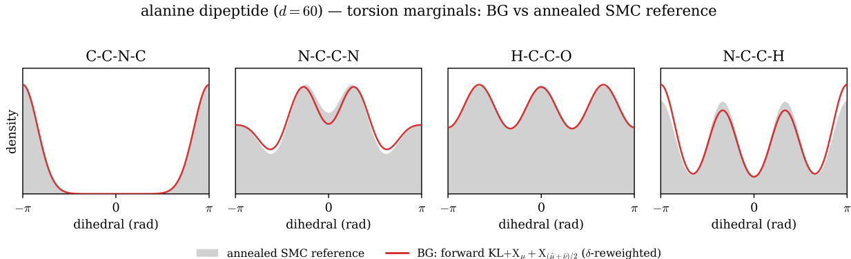
Figure 20: Alanine dipeptide torsion marginals of the BG deliverable (red) against a converged molecular-dynamics reference (grey, 2 \times 10^5 Langevin walkers). The four most multimodal proper torsions are shown; the densities are \pm\phi -symmetrised, the achiral target having p(\phi) = p(-\phi) . The BG recovers the multimodal backbone torsions and tracks MD; the peptide-bond torsion \omega (C-C-N-C) is trans-dominant in the generator, the one torsion whose high rotation barrier also makes the uniform-init MD reference slow to converge.
