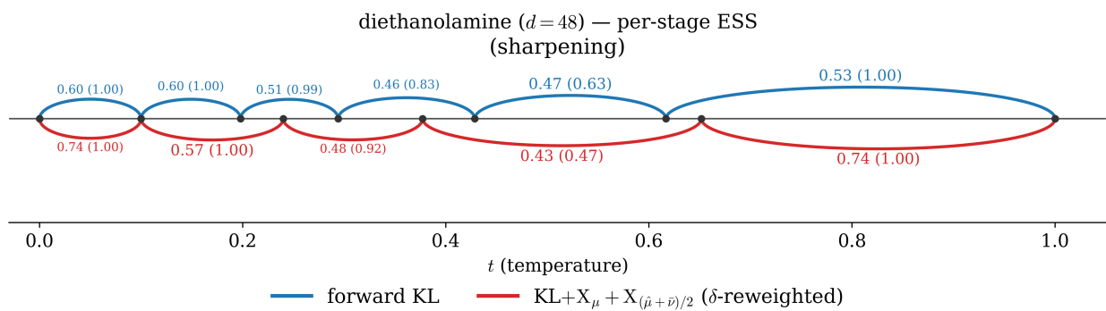
Figure 16: Diethanolamine per-stage ESS as annealing-ladder arcs (sharpening schedule): forward KL above the axis (blue), \text{KL} + X_\mu + X_{(\bar{\mu} + \bar{\nu})/2} , \delta -reweighted, below (red). Each arc is an accepted stage; the apex label is that stage's validation ESS, with the sharpening ESS in parentheses.
