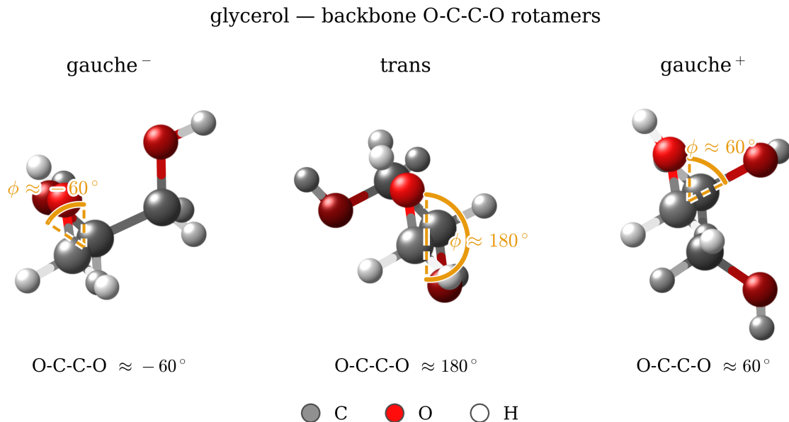
Figure 14: Typical glycerol configurations at the three states of the backbone O-C-C-O torsion: gauche − ( -60^\circ ), trans ( 180^\circ ), gauche + ( +60^\circ ). The gold arc marks the dihedral \phi ; ball-and-stick (C grey, O red, H white).
