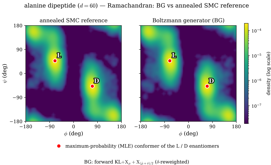
Figure 22: Alanine dipeptide Ramachandran (\phi, \psi) , shared log-density scale: the BG deliverable (right) against the annealed SMC reference (left). Red dots mark the maximum-probability conformer of each enantiomer (L at \phi < 0, \psi > 0 ; D at \phi > 0, \psi < 0 ). Both panels populate the same backbone basins with the (\phi, \psi) \rightarrow (-\phi, -\psi) point symmetry: the achiral vacuum force field makes the L- and D-enantiomers isoenergetic, and the generator, carrying no chirality constraint, samples both (Section 6.4.3).
