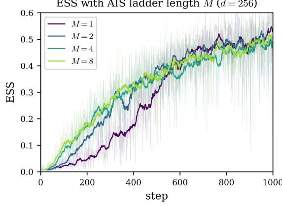
Figure 6: ESS trajectory across training steps for the mixture loss \text{KL} + X_\mu + X_{(\hat{\mu} + \bar{\nu})/2} on the product multi-well at d = 256 , as the AIS ladder length M that builds the \mu -surrogate is varied over \{1, 2, 4, 8\} . Faint lines are the raw per-step ESS; bold lines are a moving average.
