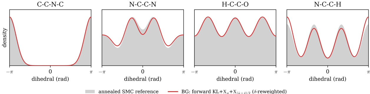
Figure 20: Alanine dipeptide torsion marginals of the BG deliverable (red) against a converged molecular-dynamics reference (grey, 2 \times 10^5 Langevin walkers). The four most multimodal proper torsions are shown; the densities are \pm\phi -symmetrised, the achiral target having p(\phi) = p(-\phi) . The BG recovers the multimodal backbone torsions and tracks MD; the peptide-bond torsion \omega (C-C-N-C) is trans-dominant in the generator, the one torsion whose high rotation barrier also makes the uniform-init MD reference slow to converge.
