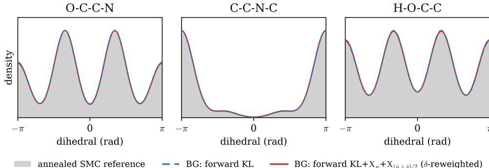
Figure 18: Diethanolamine torsion marginals of both generators against a converged molecular-dynamics reference (grey, 2 \times 10^5 Langevin walkers): forward KL (blue) and \text{KL} + X_\mu + X_{(\hat{\mu} + \bar{\nu})/2} , \delta -reweighted (red), both sharpened with the cap annealed to e_{\text{cap}} = 200 kJ/mol. Both recover the multimodal backbone torsions and track the MD reference.
