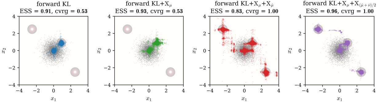
Figure 4: Sparse target. Columns show forward KL, \text{KL}+\text{X}_\mu , \text{KL}+\text{X}_\mu+\text{X}_{\hat{\mu}} , and \text{KL}+\text{X}_\mu+\text{X}_{(\hat{\mu}+\bar{\nu})/2} , with the learned pushforward overlaid on the target energy; panel titles report final ESS and coverage, and gray points show the source. The first two objectives cover the central pair but miss the two remote modes. The \hat{\mu} -only objective restores the remote modes with visible mass between components, whereas the equal mixture covers all four modes with less intermodal mass and higher ESS.
