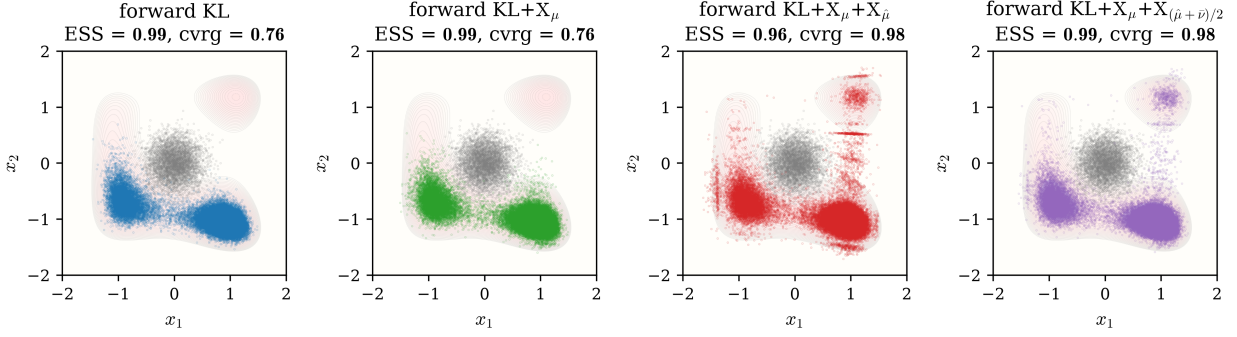
Figure 2: Three-Well target. From left to right, the panels show forward KL, \text{KL} + X_\mu , \text{KL} + X_\mu + X_{\hat{\mu}} , and \text{KL} + X_\mu + X_{(\hat{\mu} + \bar{\nu})/2} . Each panel overlays the learned pushforward on the target energy and reports final ESS and coverage; gray points show the source. Forward KL and \text{KL} + X_\mu represent the two favored wells but miss the suppressed third well. Both objectives weighted by \hat{\mu} place samples in all three wells, and the equal mixture retains the higher ESS of the two mode-complete fits.
