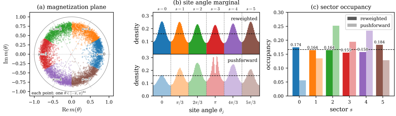
Figure 7: Structure of the cold clock measure (31) at D = 64 , displayed on 10^6 reweighted samples: fresh source draws advanced through the trained ladder by the map–reweight–resample step (v), X-regularized loss at B = 10^4 . (a) Global magnetization m(\theta) , colored by sector index s(\theta) , 1500 points per sector: the measure splits into p = 6 equivalent sectors with mean |m| = 0.73 , well developed yet contiguous through the disordered center, so every training batch touches all sectors and the multimodality is soft. (b) Site-angle marginal: the anisotropy locks each site to the six clock angles 2\pi k/6 ; dashed lines bound the six wells, colored as in (c), and the black line marks the uniform density 1/(2\pi) ; the pushforward marginal, the maps alone without reweighting, tracks the reweighted one closely. (c) Sector occupancy of reweighted and pushforward samples, the black line marking the uniform occupancy 1/6 : all six sectors are populated, and reweighting corrects the occupancy bias from total variation 0.18 to 0.025, uniform to \pm 0.02 per sector.
