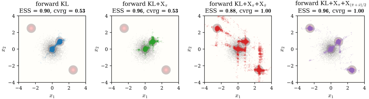
Figure 5: Sparse target. Columns show forward KL, \text{KL}+\text{X}_\pi , \text{KL}+\text{X}_\pi+\text{X}_{\hat{\pi}} , and \text{KL}+\text{X}_\pi+\text{X}_{(\hat{\pi}+\bar{\nu})/2} , with the pushforward samples overlaid on the target energy; panel titles report final ESS and coverage, and gray points show the source.
