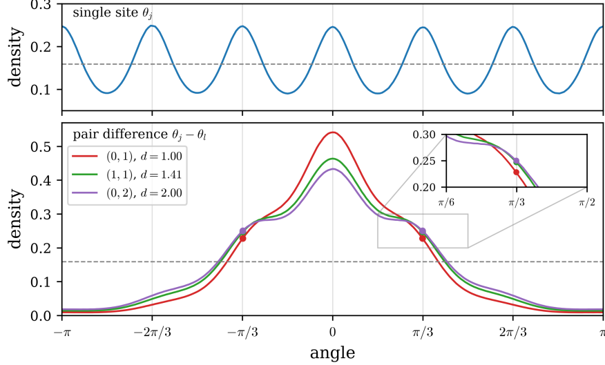
Figure 7: Angle densities from 2 \times 10^6 fresh samples advanced through the trained B = 2000 \text{KL} + \text{X}_\mu + \text{X}_{(\hat{\mu} + \bar{v})/2} stage sequence by map, reweighting, resampling, and MALA. The upper panel is the single-site marginal. The lower panel gives pair differences at offsets (0, 1), (1, 1), and (0, 2); dots and the inset resolve the one-clock-step angle \pi/3 . Dashed lines show the uniform density.
