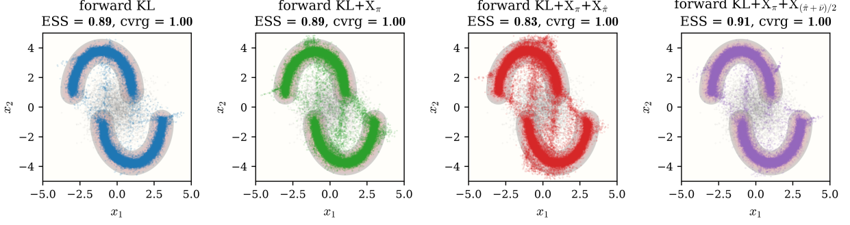
Figure 2: Two-Moon target. Columns, from left to right, are forward KL, KL+ X_\pi , KL+ X_\pi+X_{\hat{\pi}} , and KL+ X_\pi+X_{(\hat{\pi}+\bar{\nu})/2} . Each panel overlays the pushforward samples on the target energy and reports final ESS and coverage. Gray points show the source.
