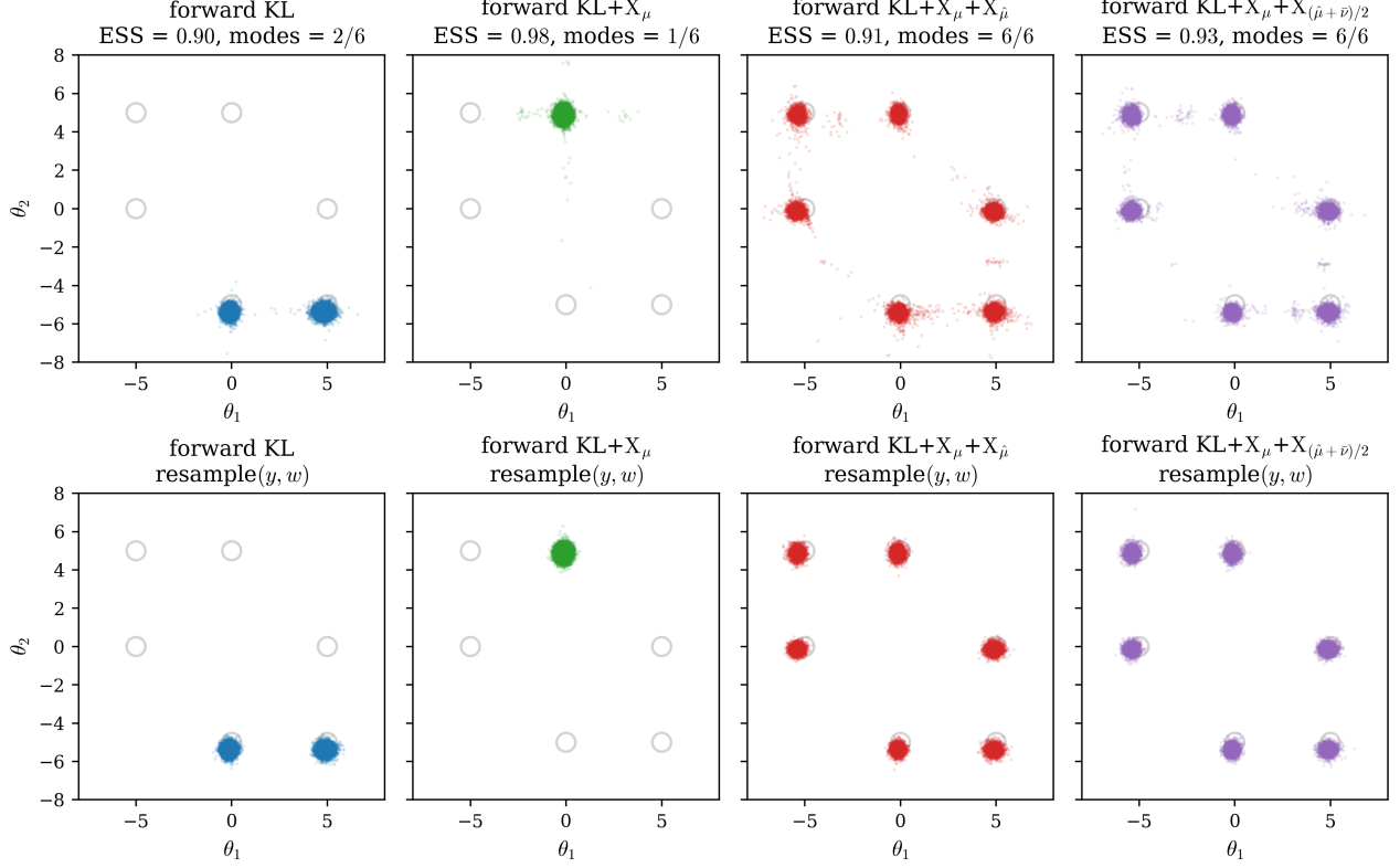
Figure 5: Sensor-array posterior, pushforward positions projected onto (\theta_1, \theta_2) . Row 1: raw pushforward y = G^{-1}(x) ; Row 2: resample( y, w ) with Langevin rejuvenation. Columns left to right: forward KL, KL+ X_\mu , KL+ X_\mu+X_{\hat{\mu}} , KL+ X_\mu+X_{(\hat{\mu}+\bar{v})/2} . Light-gray circles mark the six permutation mode centers; each title reports the final ESS and the modes found out of six. Forward KL and KL+ X_\mu collapse onto 1-2 modes at high ESS, while X_{\hat{\mu}} and the mixture fill all six.
