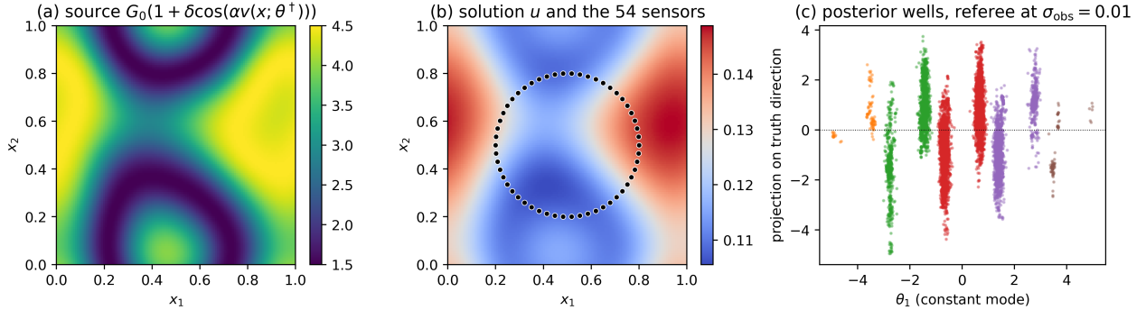
Figure 11: The screened Poisson inverse problem. (a) The true source G_0(1 + \delta \cos(\alpha v(x; \theta^\dagger))) on [0, 1]^2 . (b) The corresponding solution u of (35) and the 54 sensors on the ring of radius 0.3, the dotted circle, where u is observed. (c) Posterior samples from the parallel tempering referee at \sigma_{\text{obs}} = 0.01 , plotted in the constant mode \theta_1 against the projection on the truth direction and colored by the shift index n : the posterior splits into the well lattice of the cosine symmetries, the structure the ladder must reproduce with the correct relative weights.
