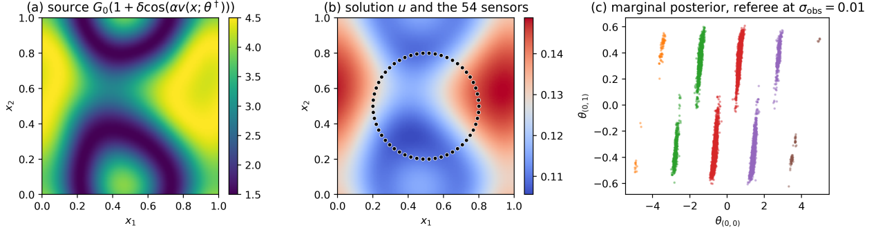
Figure 11: The screened Poisson inverse problem. (a) The true source 3(1 + \frac{1}{2} \cos(3v(\mathbf{x}; \theta^\dagger))) on [0, 1]^2 . (b) The corresponding solution u of (32) and the 54 sensors on the ring of radius 0.3, the dotted circle, where u is observed. (c) The marginal posterior in the coefficients (\theta_{(0,0)}, \theta_{(0,1)}) from the parallel tempering referee at \sigma_{\text{obs}} = 0.01 , colored by the shift index n : the posterior splits into the well lattice of the cosine symmetries.
