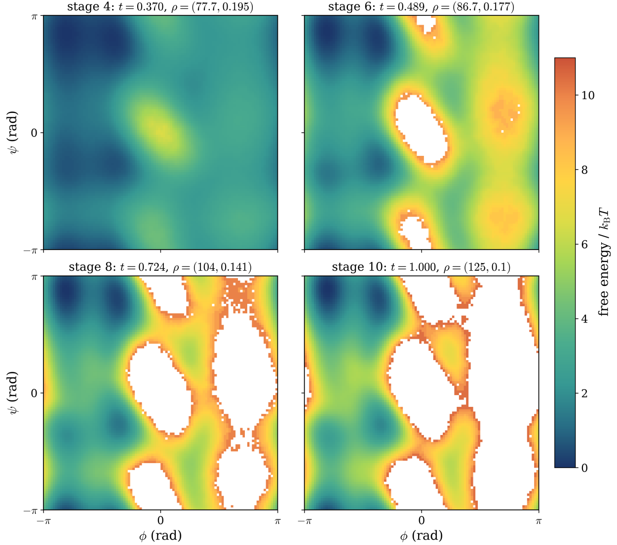
Figure 14: Alanine-dipeptide Ramachandran free-energy surfaces at accepted stages 4, 6, 8, and 10. Each panel contains 10^7 persisted inference samples after the corresponding saved-flow pushforward, resampling, rejuvenation, sharpening, and post-sharpen rejuvenation operations. The panel titles give the stage interpolation parameter and regularization value; stage 10 reaches t = 1 and \rho = (125, 0.10) . A common colorbar reports free energy relative to the observed minimum in units of k_B T .
