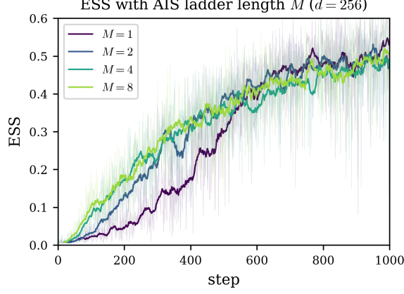
Figure 4: ESS trajectory across training steps for the mixture loss \text{KL}+X_\mu+X_{(\hat{\mu}+\bar{\nu})/2} on the product multi-well at d = 256 , as the AIS ladder length M that builds the \mu -surrogate is varied over \{1, 2, 4, 8\} . Faint lines are the raw per-step ESS; bold lines are a moving average.
