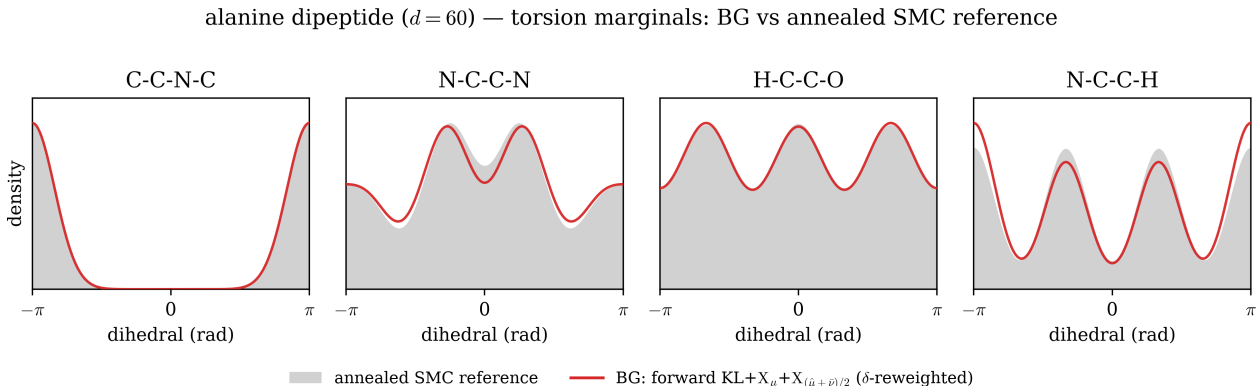
Figure 14: Alanine dipeptide torsion marginals of the BG deliverable (red) against a converged annealed SMC reference (grey). The four most multimodal proper torsions are shown; the densities are \pm\phi -symmetrised, the achiral target having p(\phi) = p(-\phi) . The BG recovers the multimodal backbone torsions and tracks the reference; the peptide-bond torsion \omega (C-C-N-C) is trans-dominant in the generator, the one torsion whose high rotation barrier also makes the uniform-init annealed SMC reference slow to converge.
