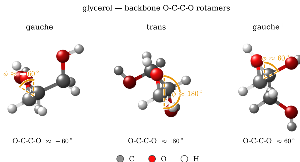
Figure S14: Typical glycerol configurations at the three states of the backbone O-C-C-O torsion: gauche − ( -60^\circ ), trans ( 180^\circ ), gauche + ( +60^\circ ). The gold arc marks the dihedral \phi ; ball-and-stick (C grey, O red, H white).
