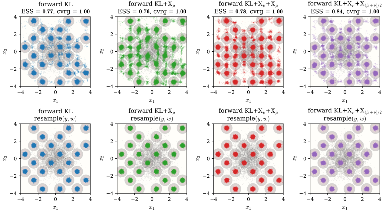
Figure S3: Chessboard target. Row 1: pushforward \mathbf{y} = G^{-1}(\mathbf{x}) . Row 2: \text{resample}(\mathbf{y}, w) with Langevin rejuvenation. Columns as in Figure S1.
