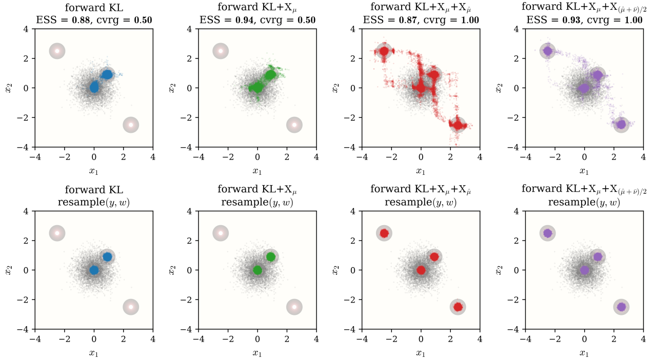
Figure S4: Sparse target. Row 1: pushforward \mathbf{y} = G^{-1}(\mathbf{x}) . Row 2: \text{resample}(\mathbf{y}, w) with Langevin rejuvenation. Columns as in Figure S1.
