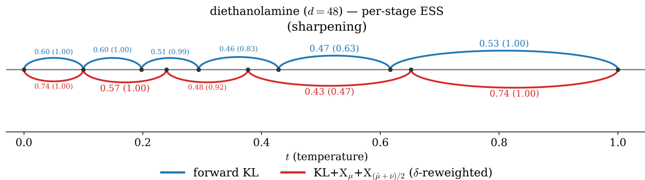
Figure S16: Diethanolamine per-stage ESS as annealing-ladder arcs (sharpening schedule): forward KL above the axis (blue), \text{KL} + X_\mu + X_{(\hat{\mu} + \bar{\nu})/2} , \delta -reweighted, below (red). Each arc is an accepted stage; the apex label is that stage's validation ESS, with the sharpening ESS in parentheses.
