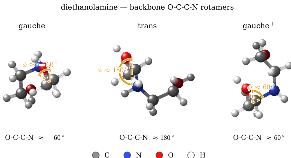
Figure S17: Typical diethanolamine configurations at the three states of a backbone O-C-C-N torsion: gauche - ( -60^\circ ), trans ( 180^\circ ), gauche + ( +60^\circ ). The gold arc marks the dihedral \phi ; ball-and-stick (C grey, N blue, O red, H white).
