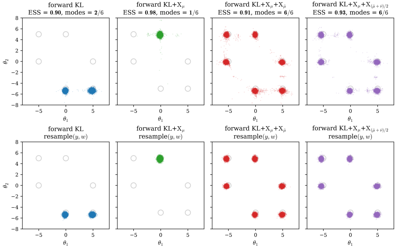
Figure S5: Sensor-array posterior, pushforward positions projected onto (\theta_1, \theta_2) . Row 1: raw pushforward \mathbf{y} = G^{-1}(\mathbf{x}) ; Row 2: \text{resample}(\mathbf{y}, w) with Langevin rejuvenation. Columns left to right: forward KL, KL+ X_\mu , KL+ X_\mu + X_{\hat{\mu}} , KL+ X_\mu + X_{(\hat{\mu}+\bar{\nu})/2} . Light-gray circles mark the six permutation mode centers; each title reports the final ESS and the modes found out of six.
