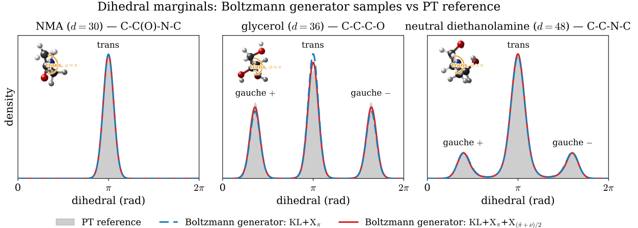
Figure 12: Dihedral marginals from the Boltzmann generator samples at t = 1 and the PT references, for NMA, glycerol, and neutral diethanolamine. Gray is the reference, dashed blue is \text{KL} + \text{X}_\pi , and solid red is \text{KLXX} ; the dashed curve is drawn over the solid one so that agreement between the two remains visible. Every density is symmetrized under \varphi \mapsto -\varphi , as the achiral targets allow, and smoothed, with the reference and both generators treated alike. The insets show a representative trans conformer.
