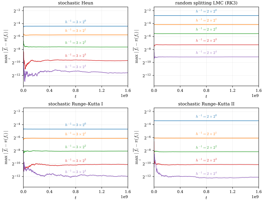
FIG. 2. Sampling error \max_i |\bar{f}_i - \pi(f_i)| of the empirical time average against the horizon, at five step sizes of equal cost per unit of time, for stochastic Heun (top left), the random splitting LMC (top right), SRK-I (bottom left) and SRK-II (bottom right). The four panels share axes.
