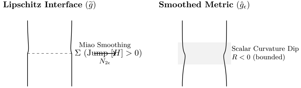
FIGURE 4. Smoothing the internal corner. The singular interface \Sigma is replaced by a smooth collar N_{2\epsilon} . The curvature "dip" inside the collar is controlled by the L^{3/2} estimate.
