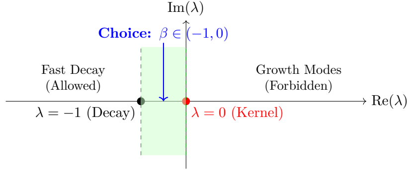
FIGURE 9. Spectral gap for the cylindrical model. Admissible weights \beta \in (-1, 0) lie strictly between the indicial roots 0 and -1 .
