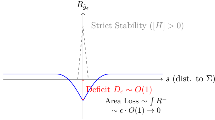
FIGURE 8. Profile of the scalar curvature during smoothing. In a separate zero-jump case (blue curve), the Dirac mass \frac{2}{\epsilon}[H] disappears, revealing the bounded quadratic deficit D_\epsilon . Because the deficit is O(1) on a collar of thickness O(\epsilon) , its L^{3/2} norm decays like \epsilon^{2/3} .
