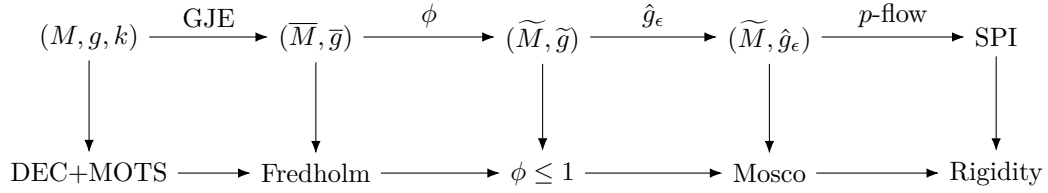
FIGURE 1. Logical flow of the proof. Geometric constructions progress along the top row, while the lower row records the analytic invariants that authorize each passage.
