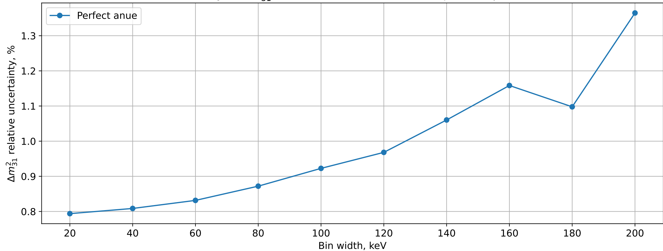
Sensitivity to \Delta m_{31}^2 as a function of bin widths of JUNO's spectrum
