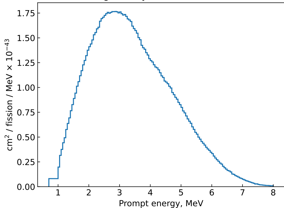
Daya Bay prompt energy spectrum weighted by IBD cross section
