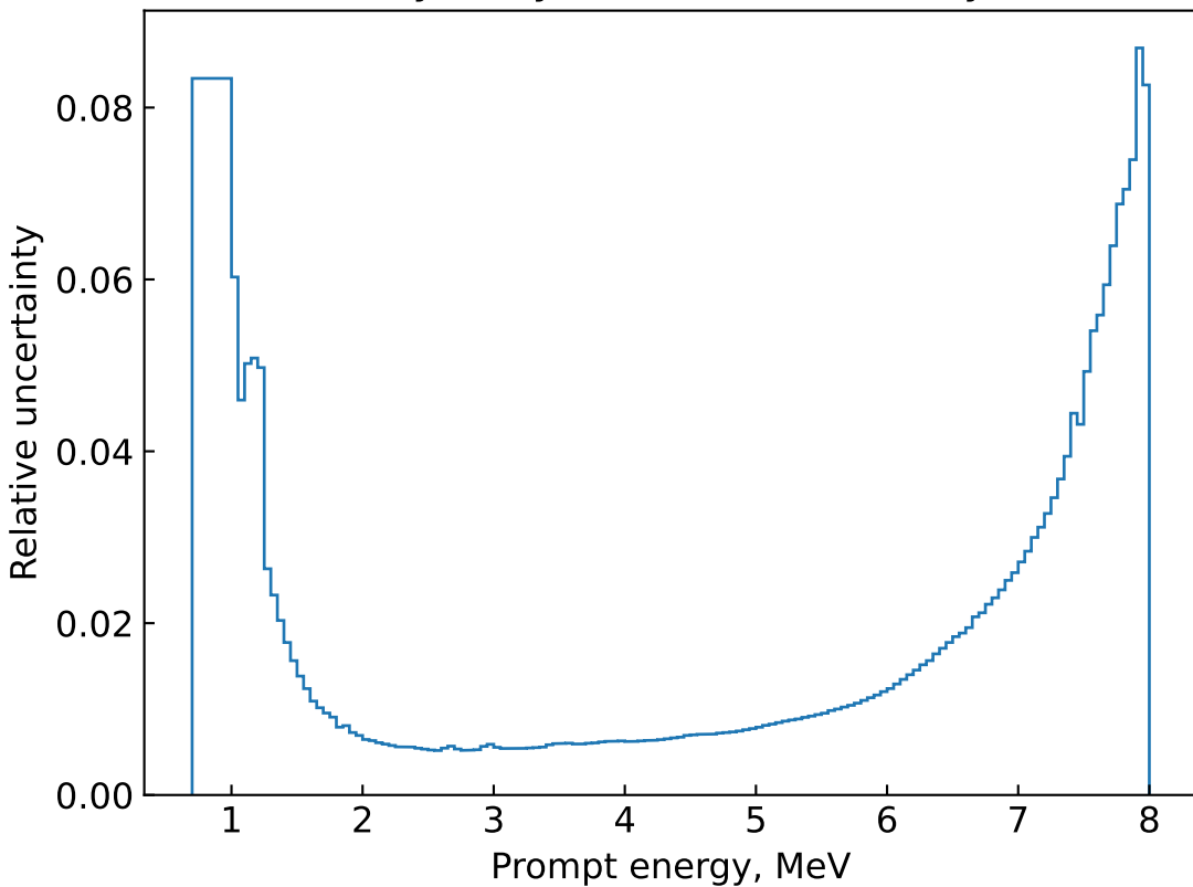
Daya Bay relative uncertainty
