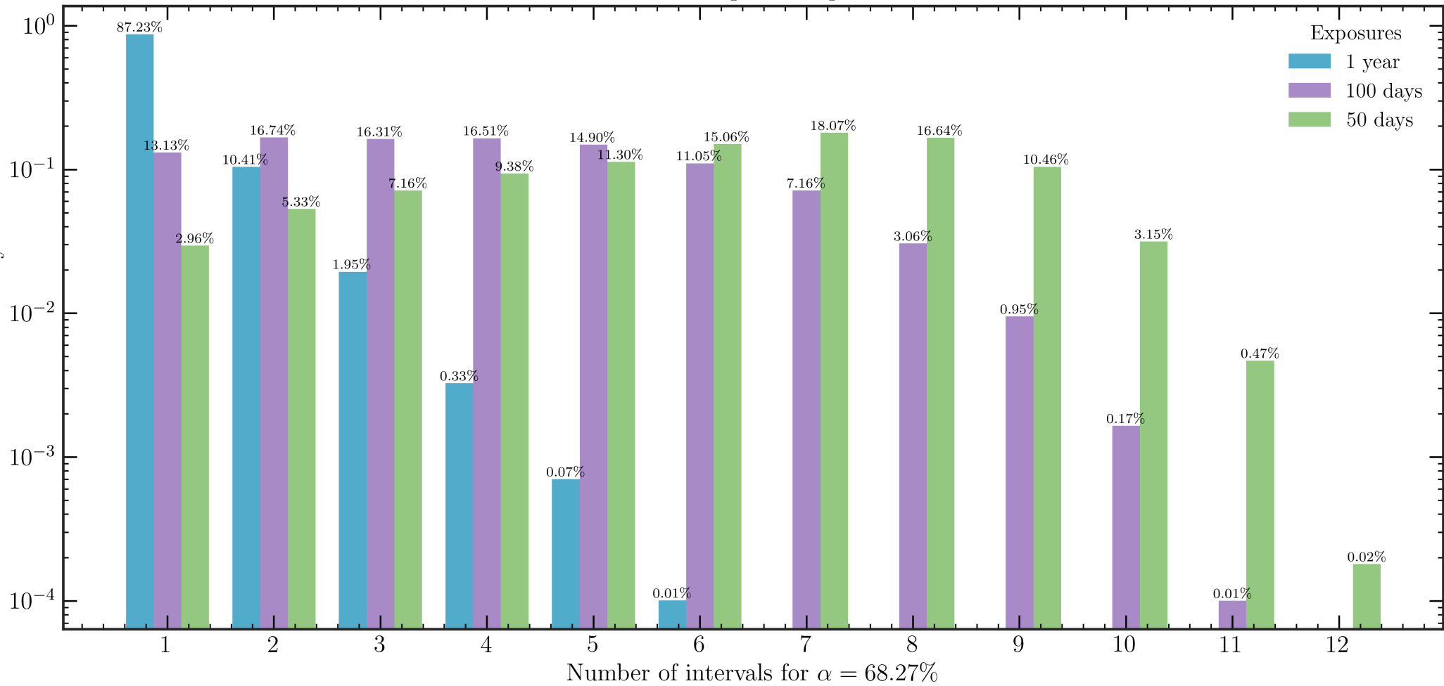
20k validation pseudoexperiments
