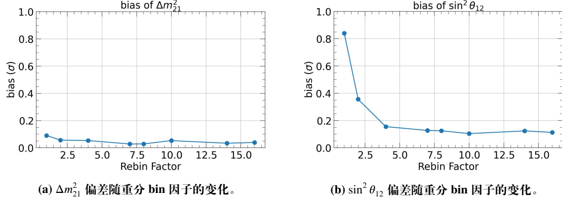
图 4-3 太阳振荡参数偏差随重分 bin 因子的演化。(a) \Delta m_{21}^2 的偏差；(b) \sin^2 \theta_{12} 的偏差。 Figure 4-3 Evolution of the bias of solar oscillation parameters as a function of the rebin factor. Panel (a) shows the bias of \Delta m_{21}^2 ; panel (b) shows the bias of \sin^2 \theta_{12} .
