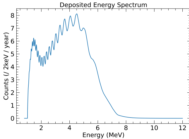
图 2-5 沉积能量能谱 Figure 2-5 Deposited energy spectrum
