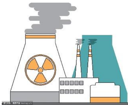
Reactor antineutrinos
