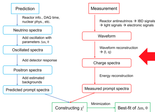
Oscillation fitting
