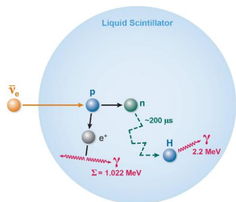
Inverted beta decay
