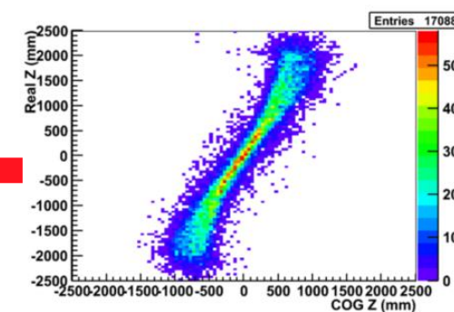
Calibration Event reconstruction ( t, Q \rightarrow E, \mathbf{r} )
