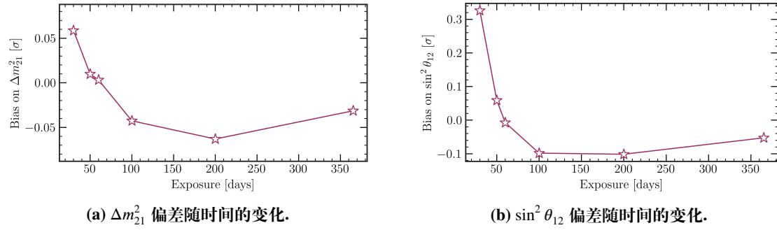
图 6-1 太阳振荡参数偏差随曝光时间的演化。(a) \Delta m^2_{21} 的偏差；(b) \sin^2 \theta_{12} 的偏差。 Evolution of the bias of solar oscillation parameters as a function of exposure time. Panel (a) shows the bias of \Delta m^2_{21} ; panel (b) shows the bias of \sin^2 \theta_{12} .
