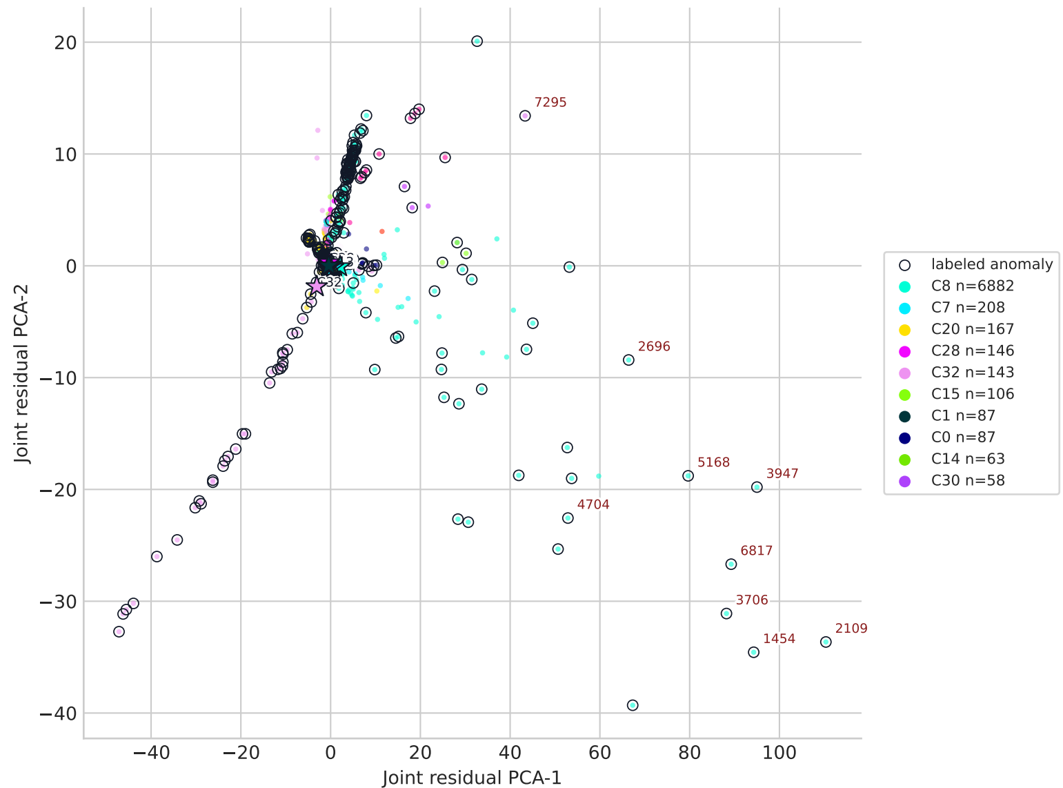
weibo trial 0: trained residual communities
