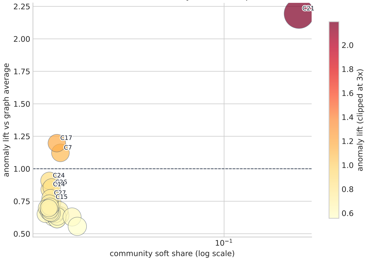
weibo trial 1: community mass-risk profile
