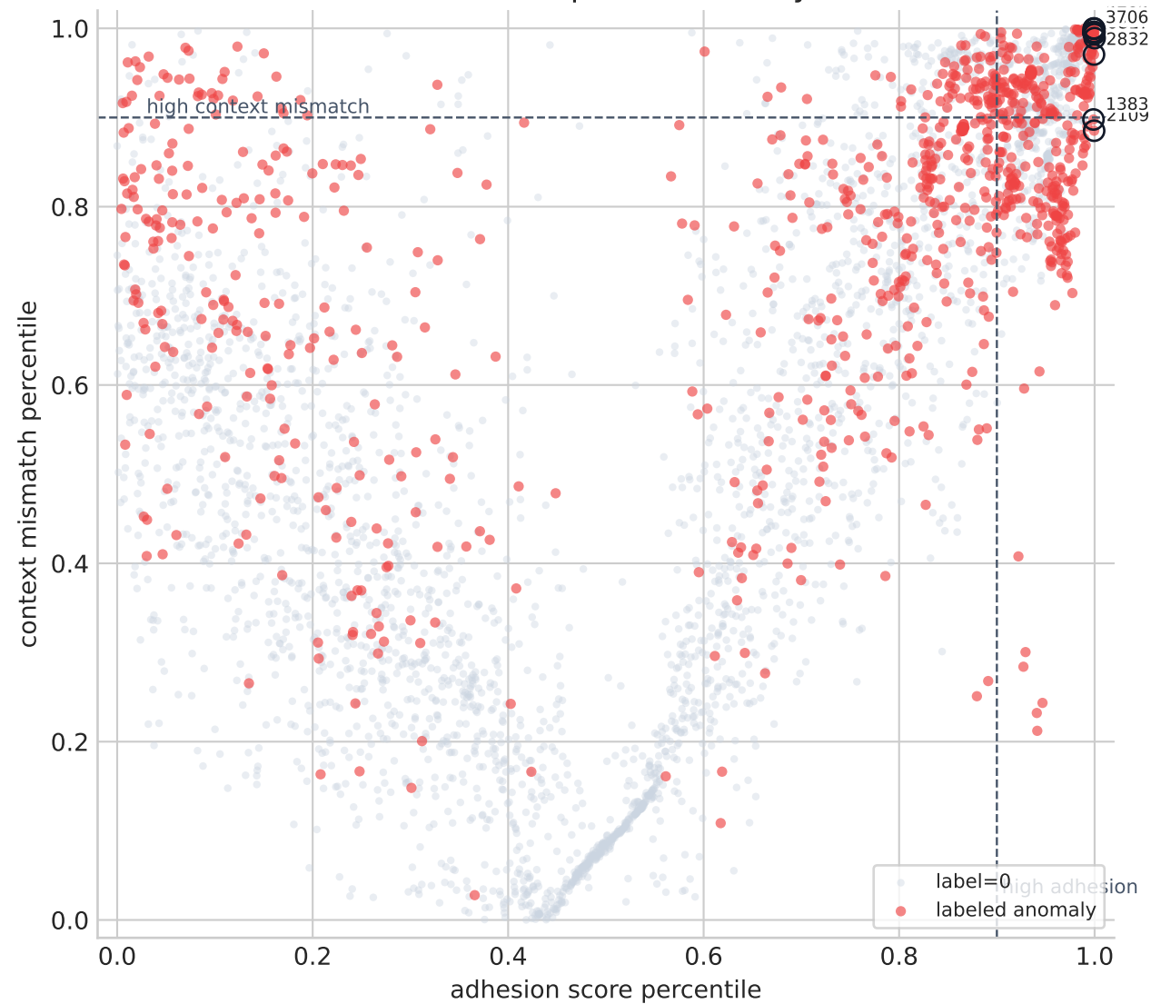
weibo trial 1: decomposed anomaly evidence
