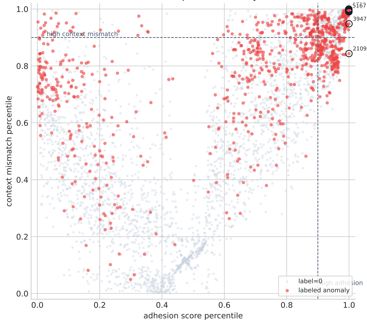
weibo trial 2: decomposed anomaly evidence
