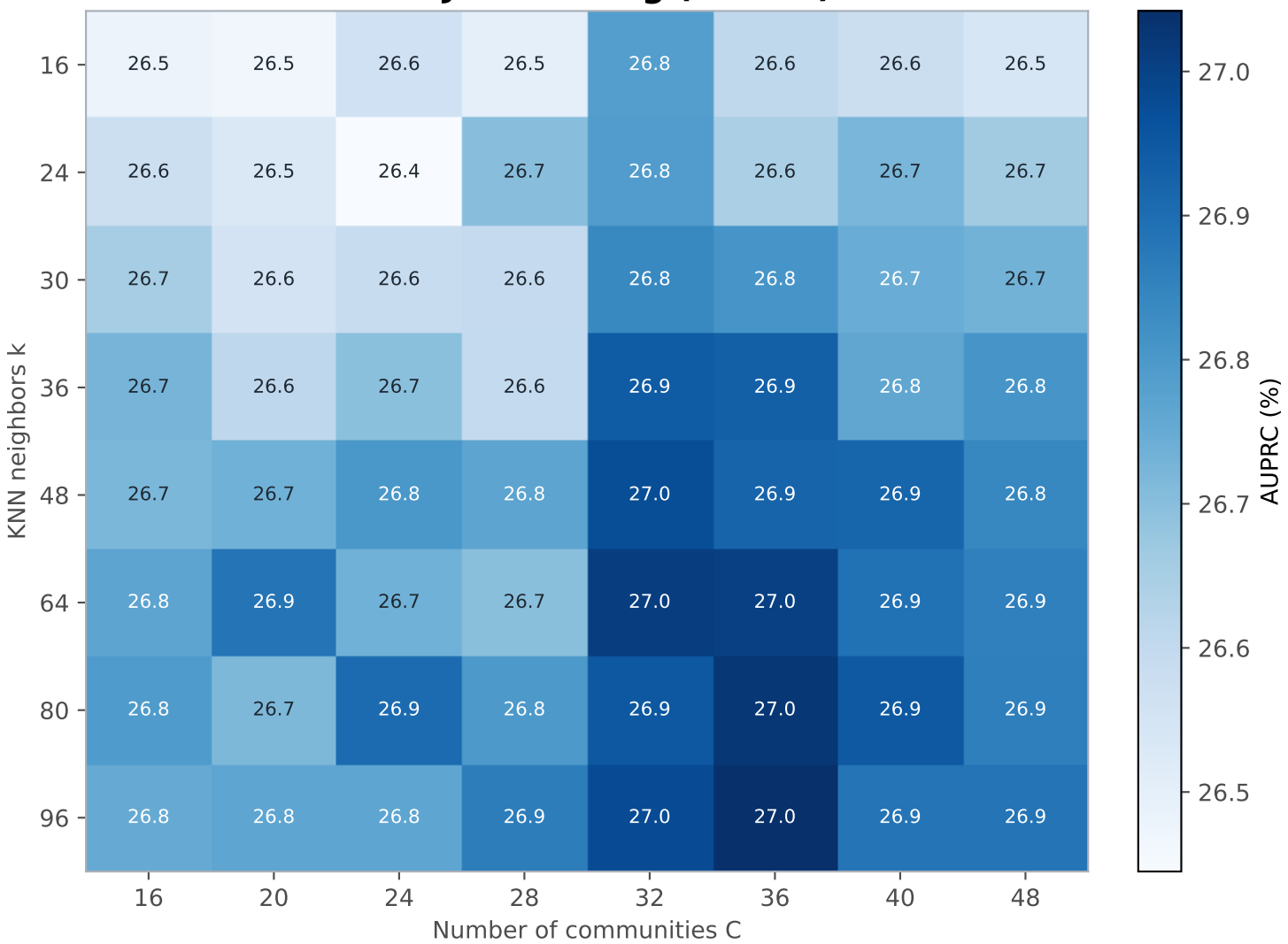
K x C Joint Tuning (AUPRC)
