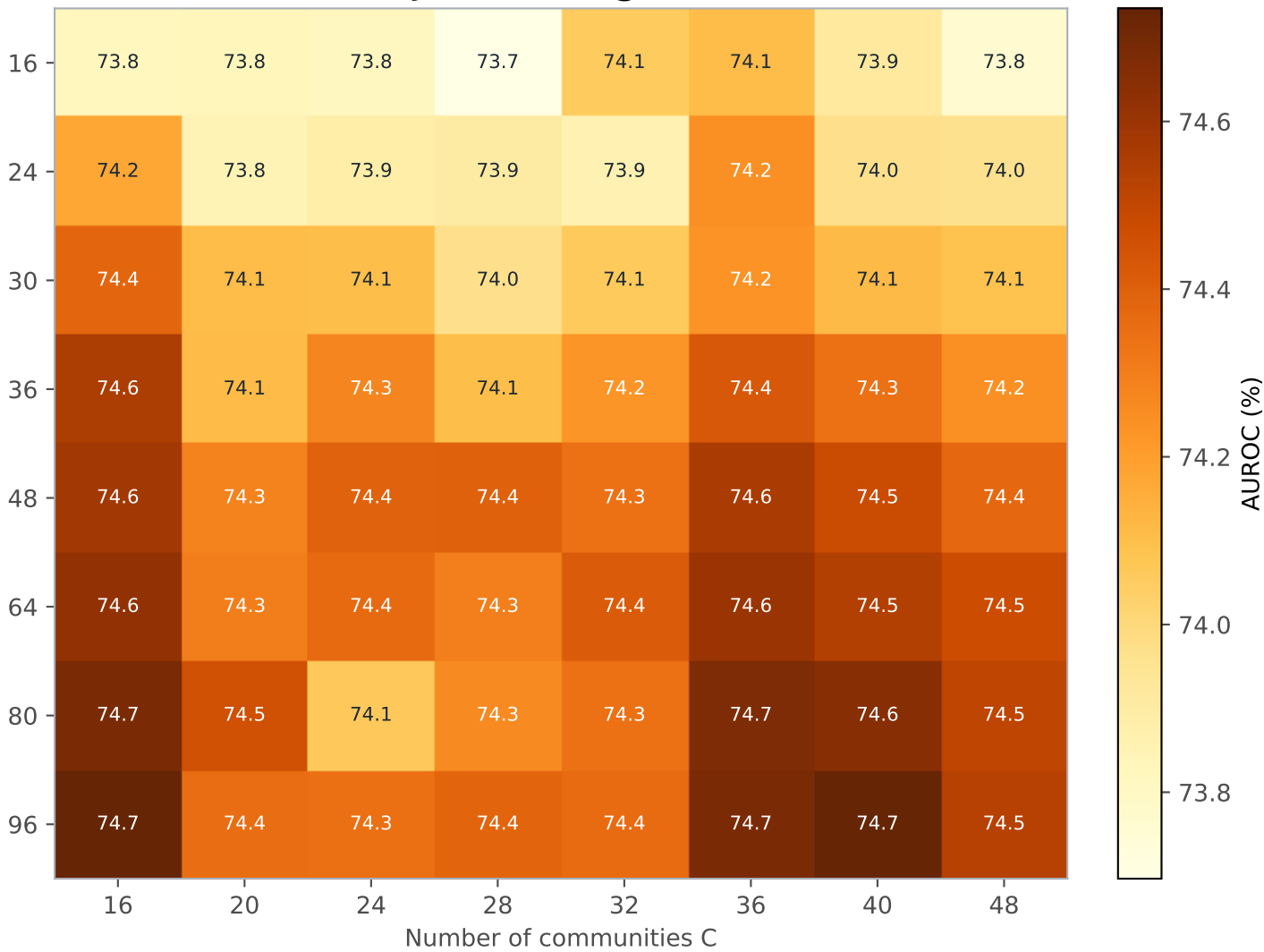
k x C Joint Tuning (AUROC)
