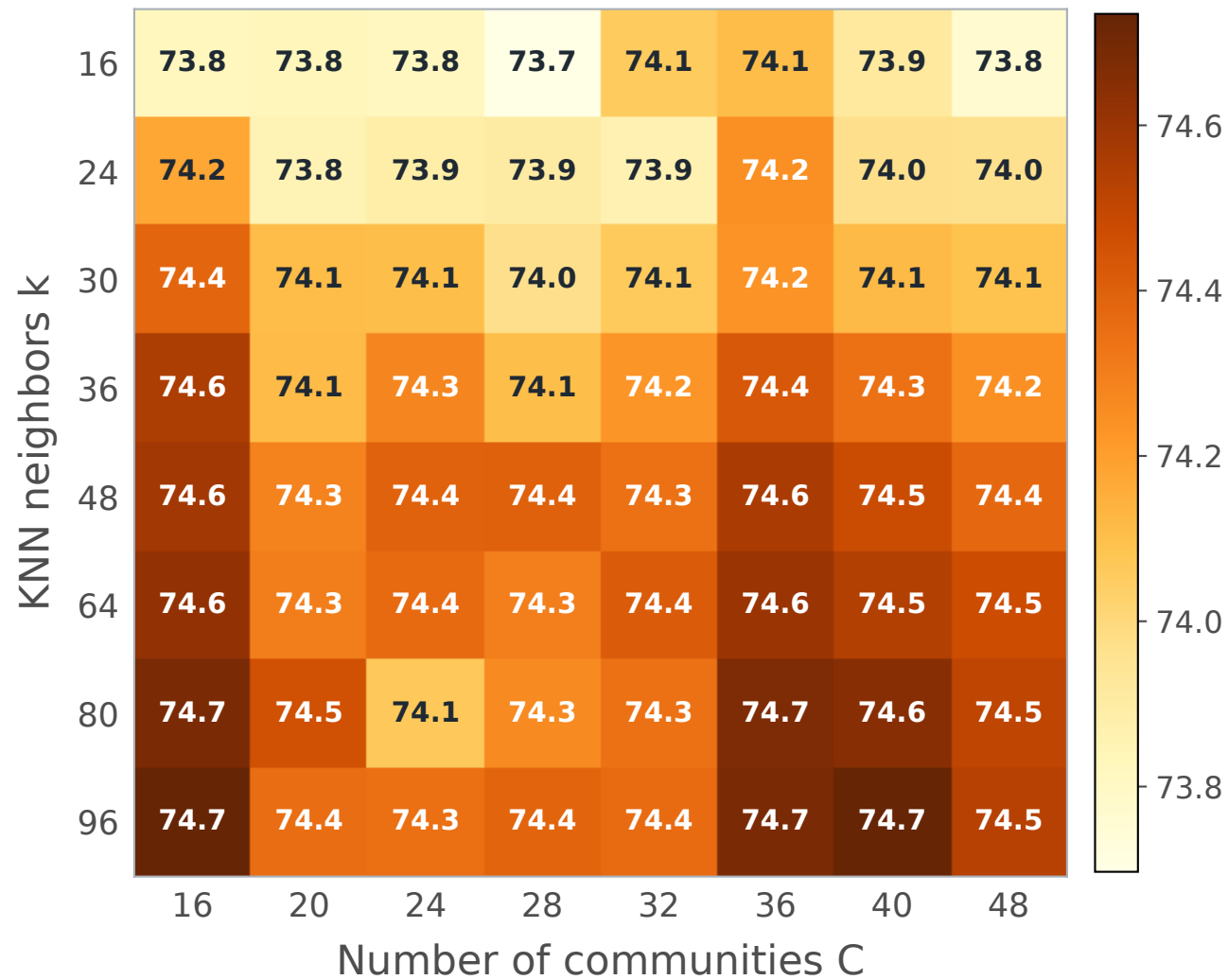
(a) AUROC
