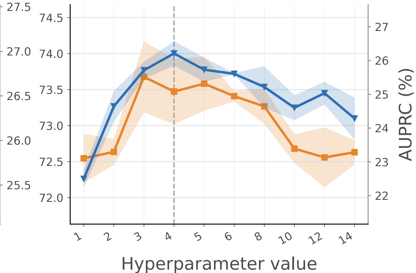
(b) Propagation depth L
