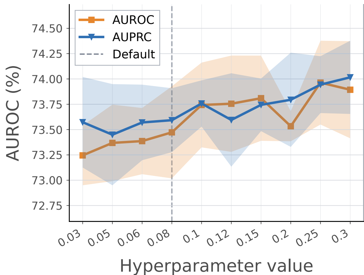
(a) Similarity temperature \tau_s
