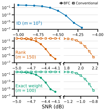
(b) Noisy channel
