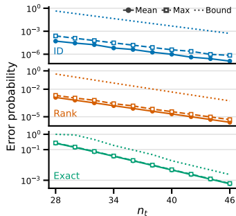
(a) Noiseless channel
