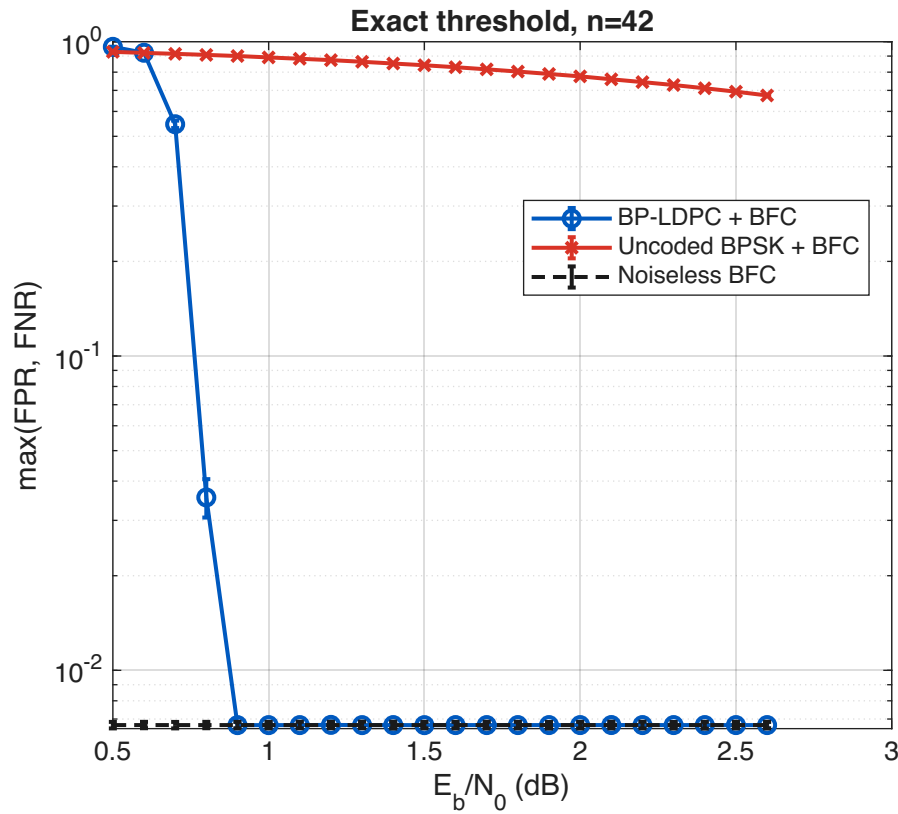
BP-LDPC/BFC waterfall with fixed-sample frame-cluster bootstrap 95% CIs
