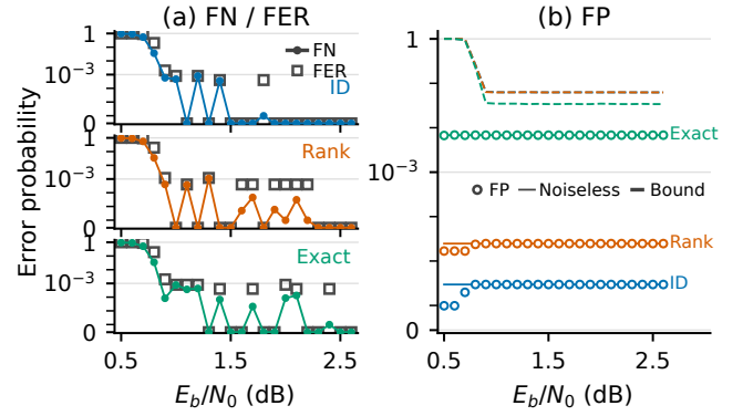
Fig. 2. Packed BFC over AWGN: (a) FN and payload FER; (b) FP, noiseless reference, and additive diagnostic.
