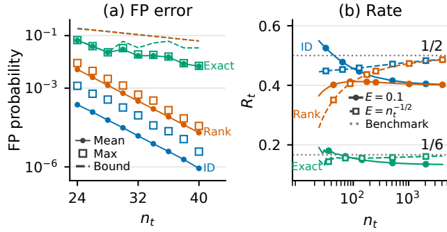
Fig. 1. Noiseless RS tagging: (a) sampled mean and maximum FP probabilities with uniform bounds; (b) finite rates and asymptotic benchmarks.
