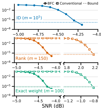
(b) Noisy channel
