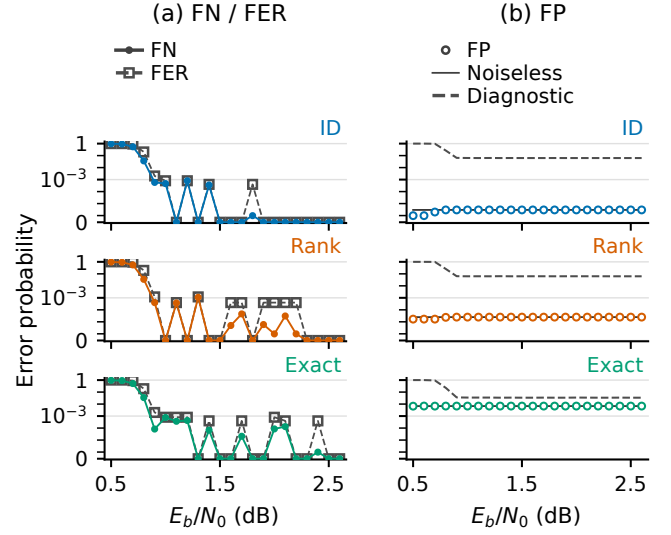
Fig. 2. Packed BFC over AWGN: (a) FN and payload FER; (b) FP, noiseless reference, and additive diagnostic.
