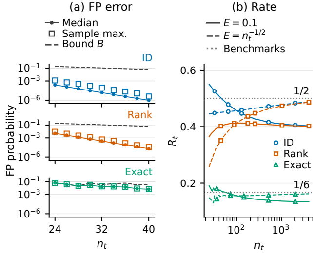
Fig. 1. Noiseless RS tagging: (a) sampled FP probabilities and uniform bounds; (b) finite rates and asymptotic benchmarks.
