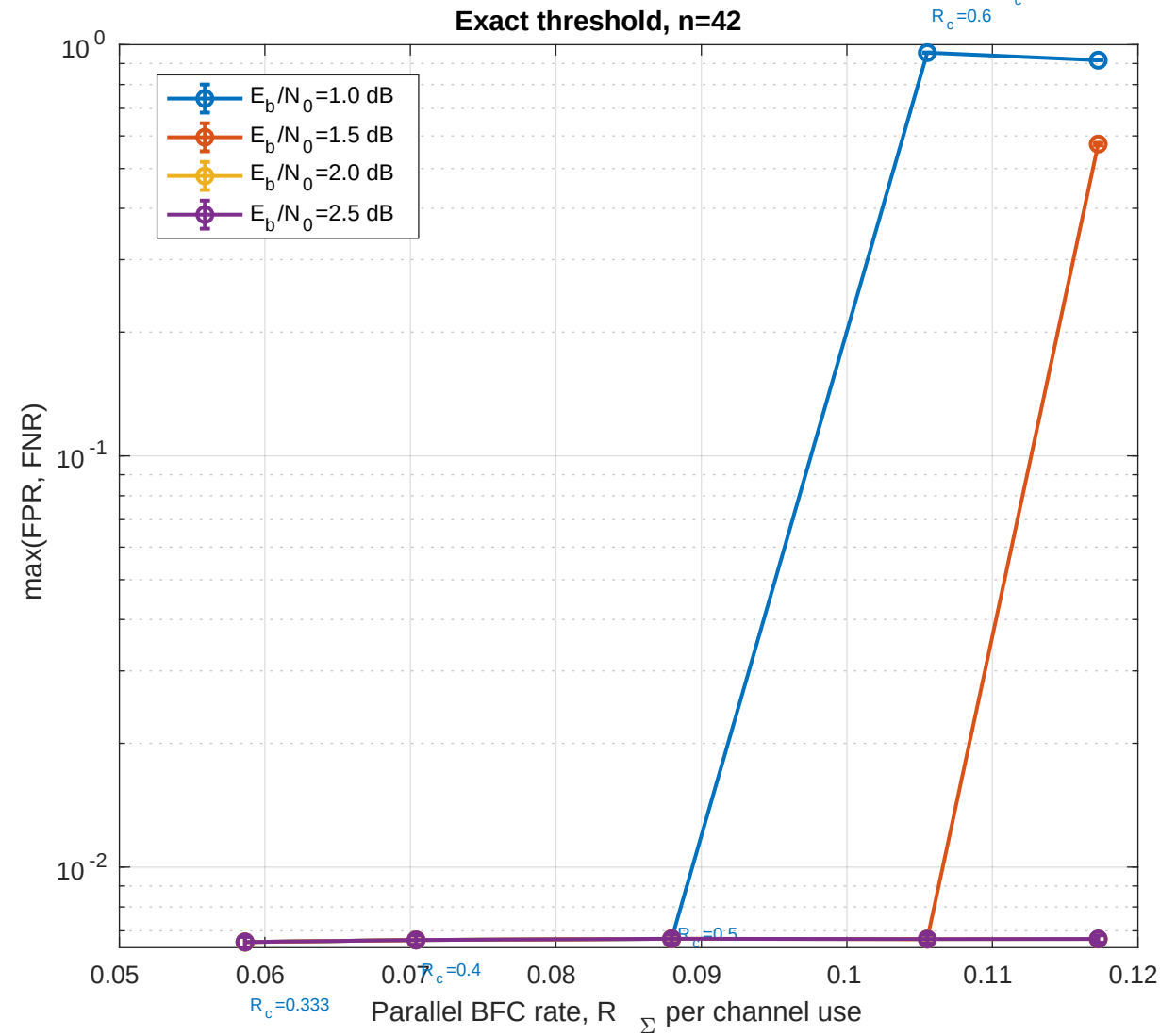
BP-LDPC fixed-sample resource-reliability tradeoff with frame-cluster bootstrap 95% CIs
