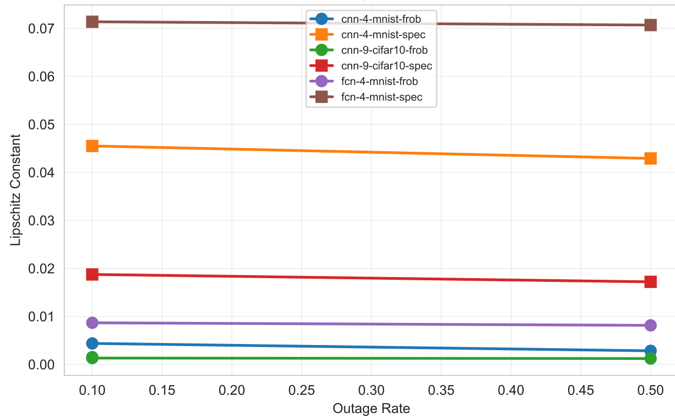
BEC: Outage Rate Effect
