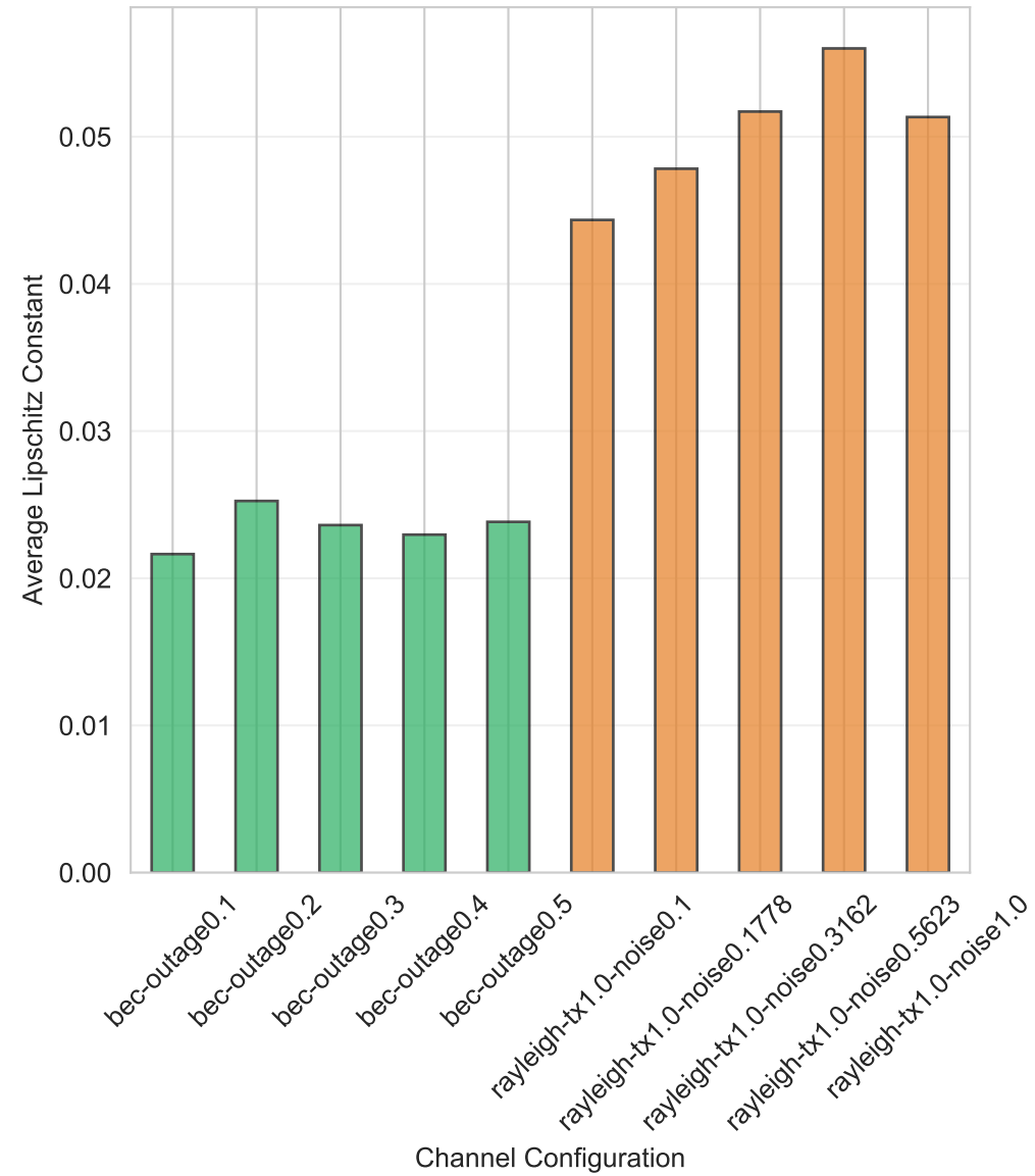
BEC (Green) vs Rayleigh (Orange) Channels
