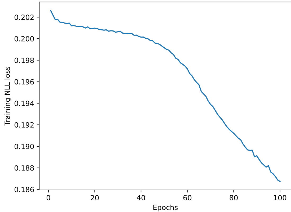
Training NLL loss fclassic, cifar10, cnn, sigma prior 0.03, pmin 1e-05, lr 0.001, momentum 0.95, kl penalty 1, dropout 0.0
