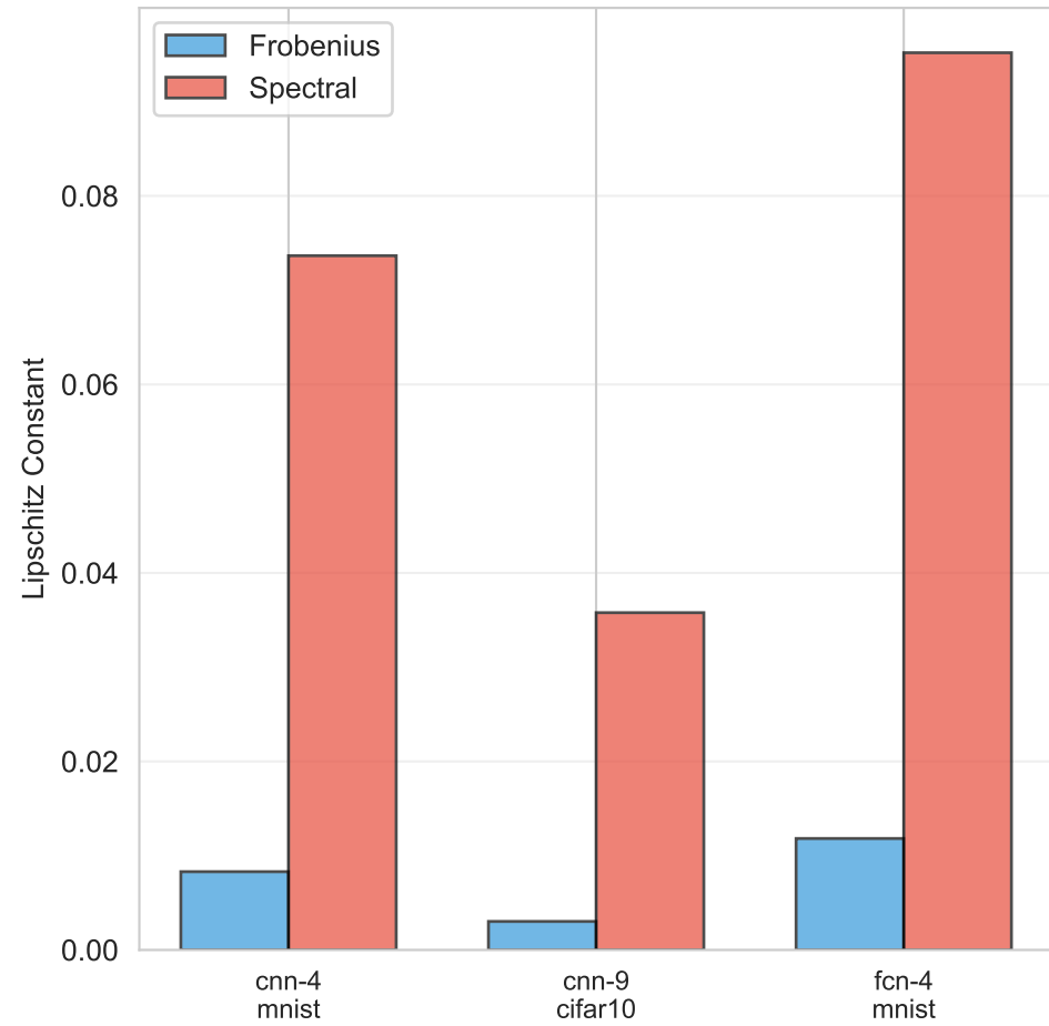
Model/Dataset vs Norm Type
