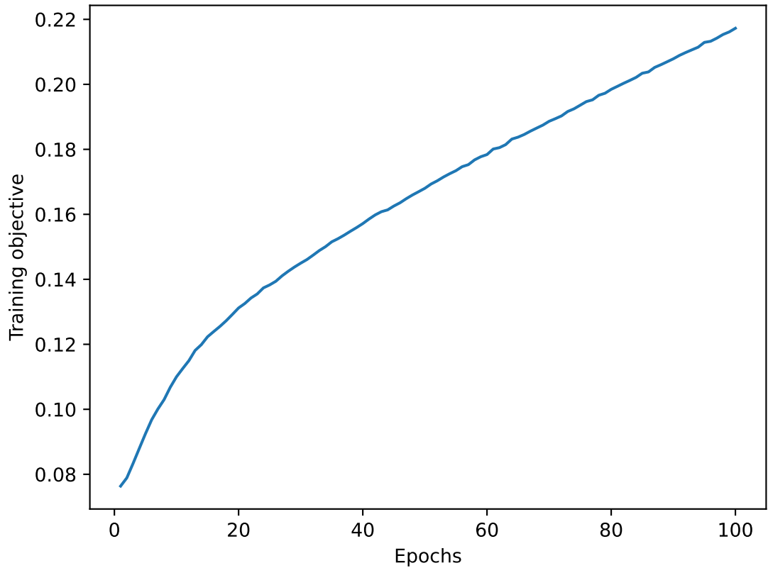
Training objective fclassic, cifar10, cnn, sigma prior 0.03, pmin 1e-05, lr 0.001, momentum 0.95, kl penalty 1, dropout 0.2
