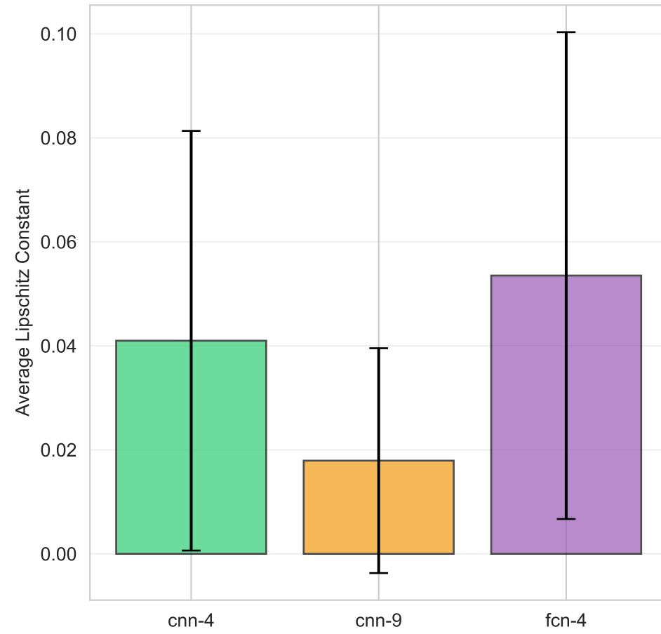
Model Architecture Comparison
