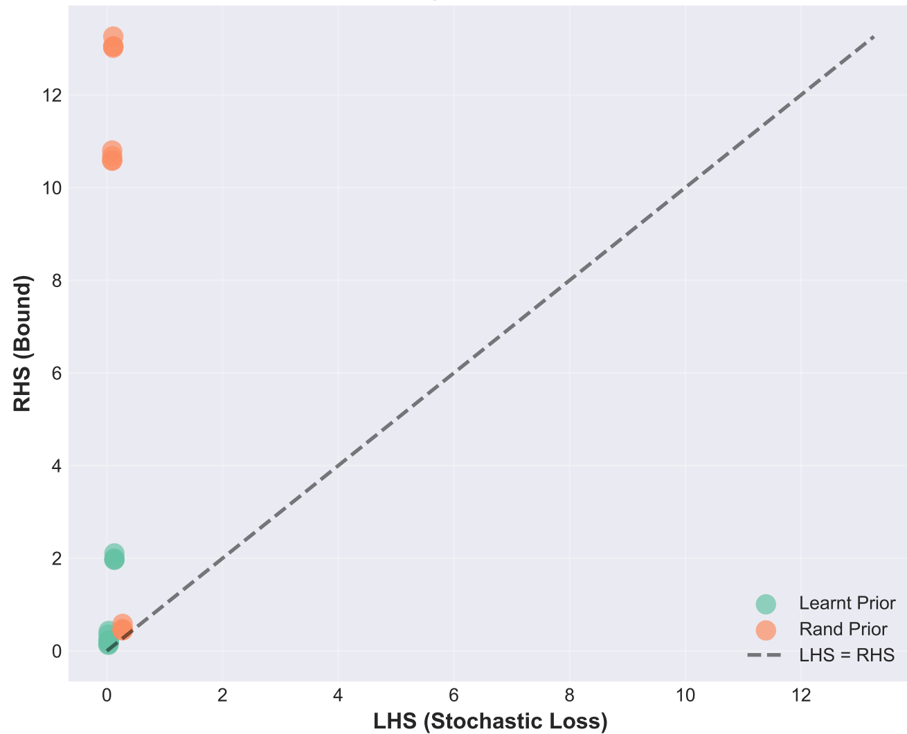
Cross-Entropy Bounds: LHS vs RHS
