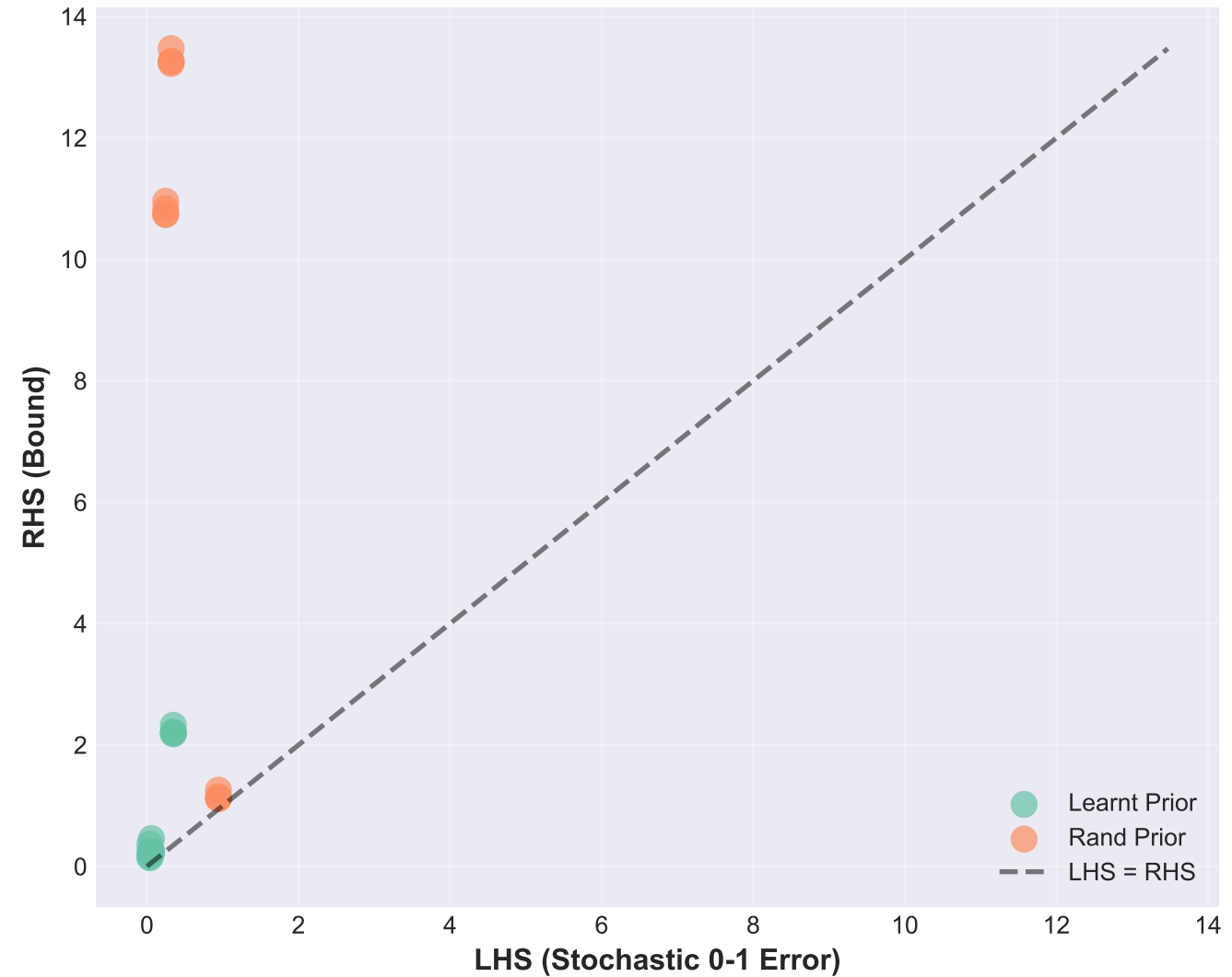
0-1 Error Bounds: LHS vs RHS
